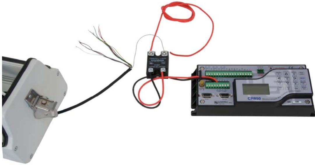
Figure B-5. Solid State Relay Connections
