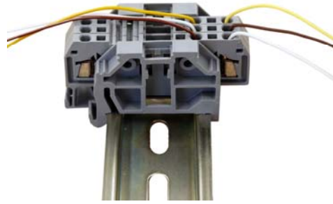
Figure 5. Remove the Screwdriver
