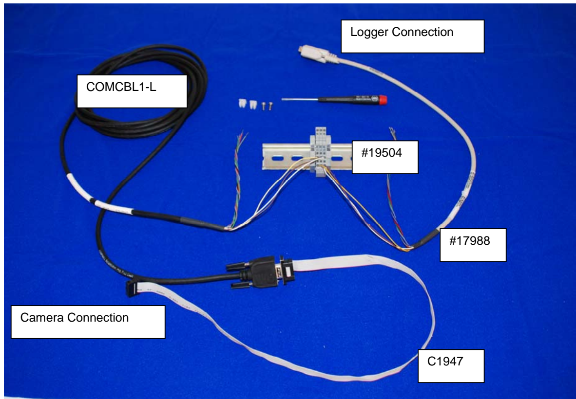
Figure 6. Camera RS-232 to RS-232 Port Connection
