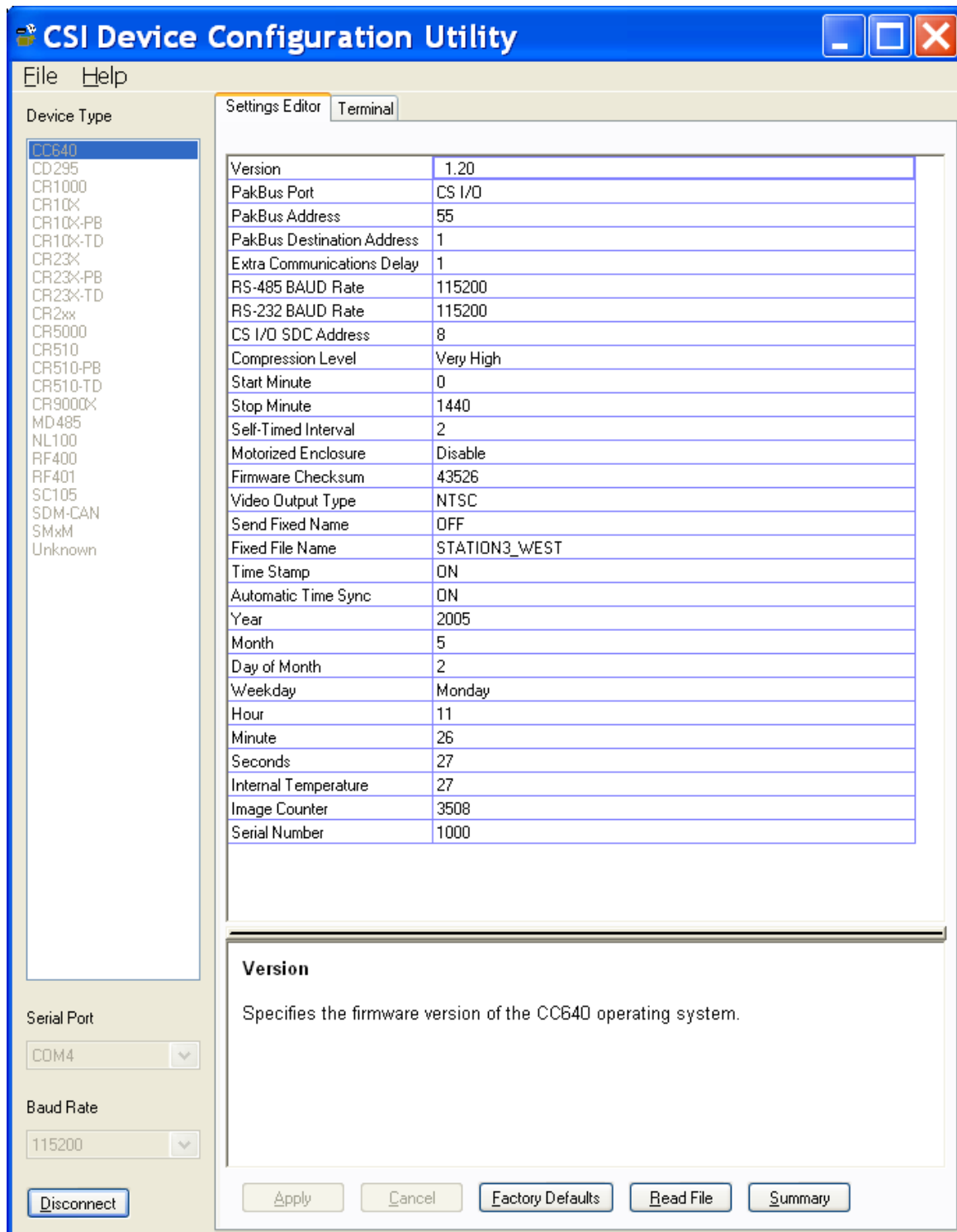
Figure 9. Device Configuration Utility Screen
