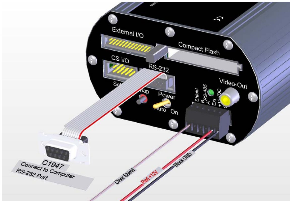
Figure 7. Connections for Configuration
