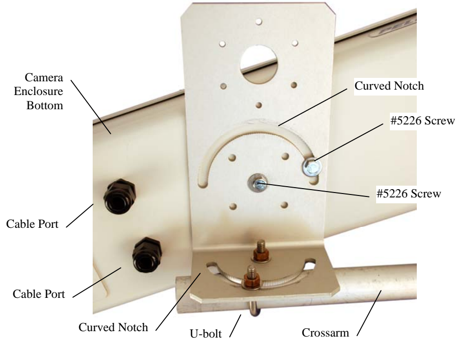
Figure 20. Camera Mount to Crossarm
