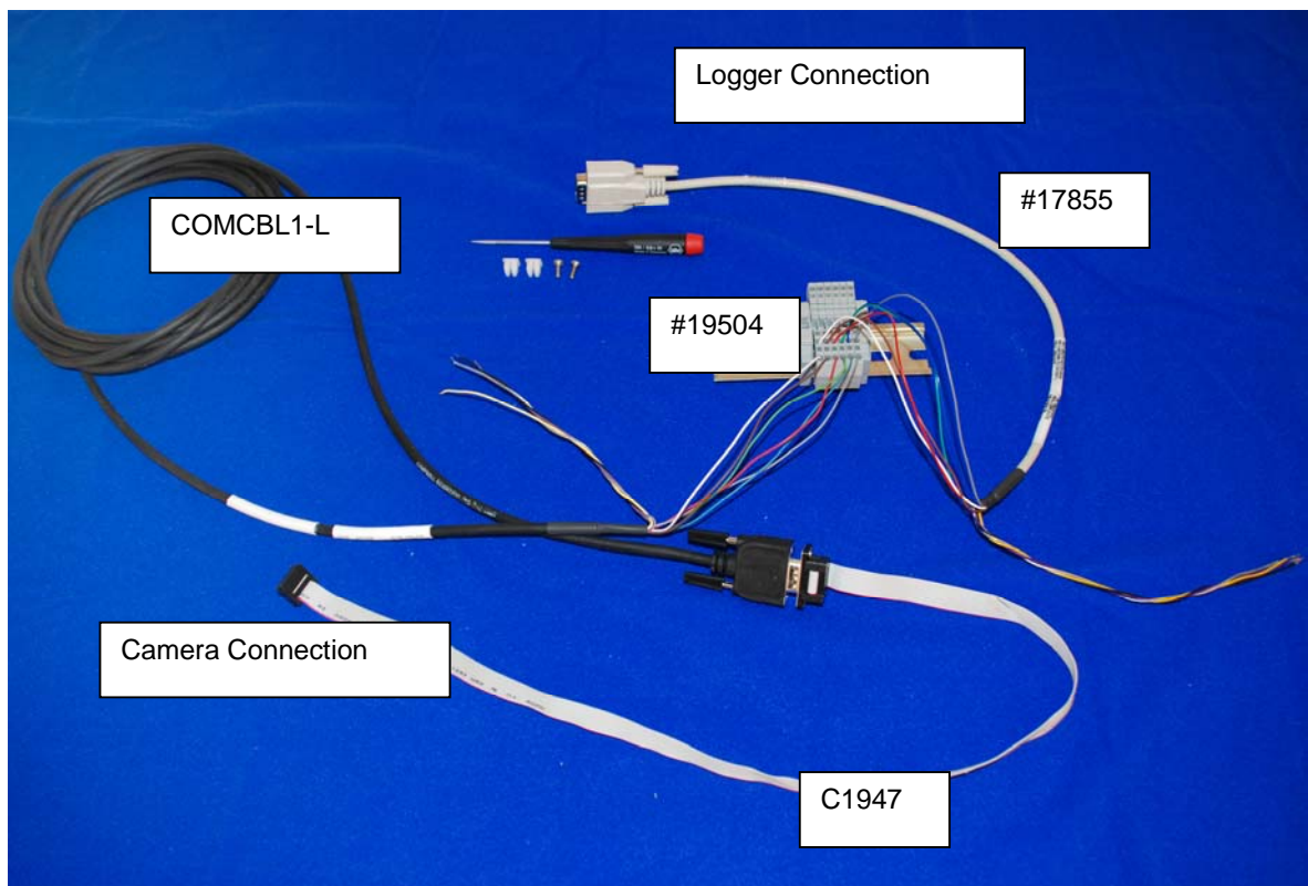
Figure 8. Camera CS/IO to Logger CS/IO Connection
